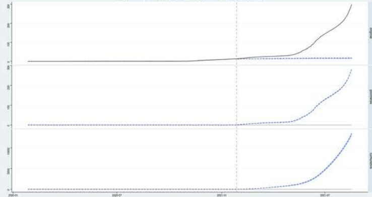
LXA: Causal Impact Plot | Total Vaccinations Per Million effect on Total Deaths Per Million
