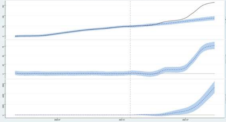
BOD: Causal Impact Plot | Total Vaccinations Per Million effect on Total Deaths Per Million
